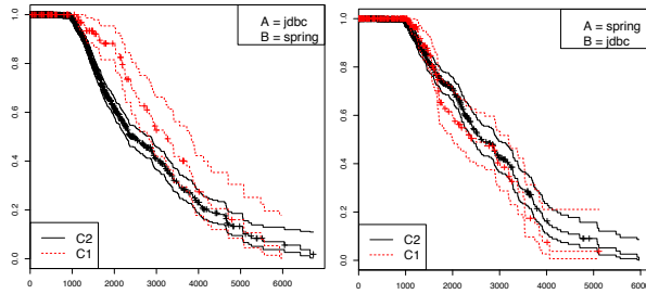
Fig. 4: Survival curves C_1 and C_2 for Spring and JDBC.
