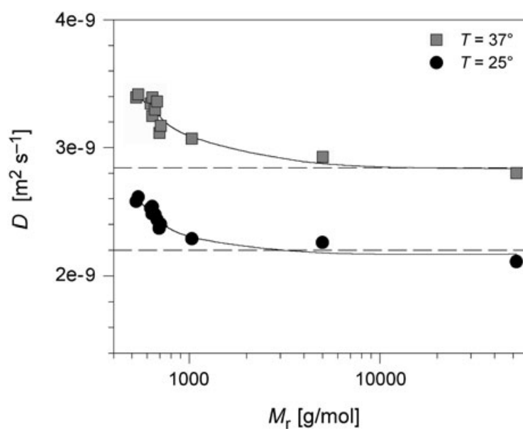
Fig. 5. Evolution of the diffusion constant with molecular weight at 25^\circ and 37^\circ . The dashed lines correspond to the diffusion coefficient of bulk \text{H}_2\text{O} .
