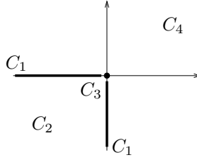
Fig. 6: Suf 2 ( \mathcal{P} )
