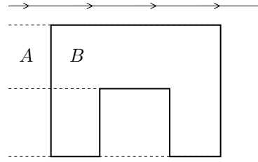
Fig. 10: Suffixes partition
