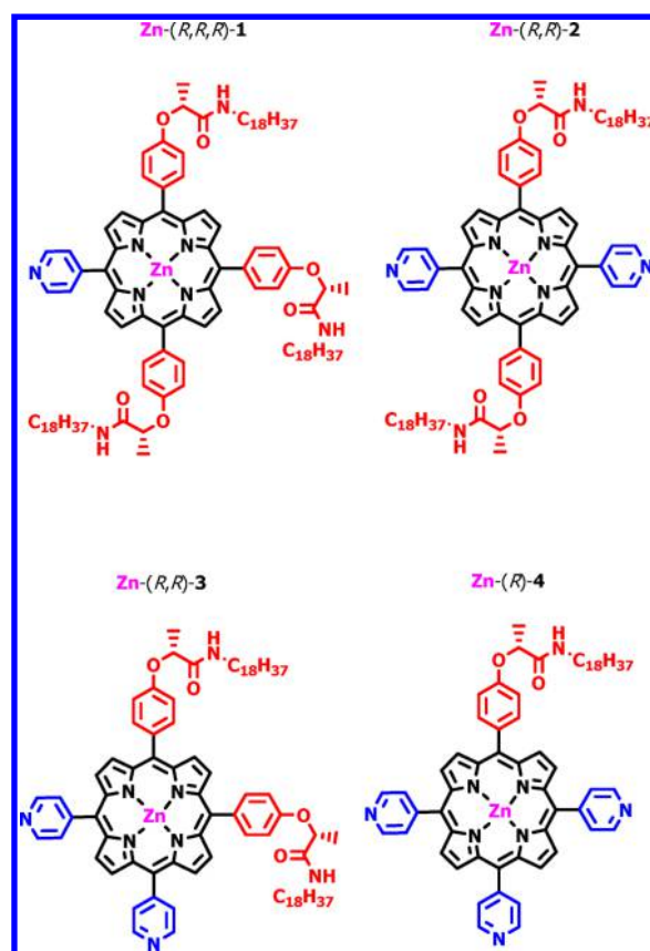
Figure 1. Target functionalized metalloporphyrins.
