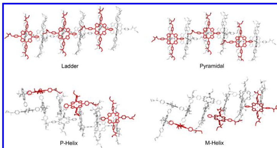
Figure 13. Proposed variants of mode A tetramer self-assembly from molecular dynamics simulations. XYZ coordinates are available in Supporting Information . One monomer per tetramer is colored in red to highlight the different submodes.
