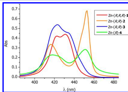
Figure 3. UV–visible absorption spectrum of compounds Zn- (R,R,R) -1, Zn- (R,R) -2, Zn- (R,R) -3 and Zn- (R) -4 at room temperature in methylcyclohexane/3% CHCl 3 (5 \mu M).
