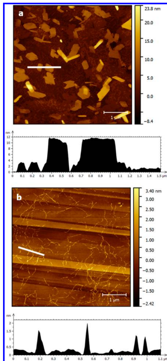
Figure 16. Tapping mode AFM images of Zn-(R,R,R)-1 cast at 0 °C on freshly cleaved HOPG.
