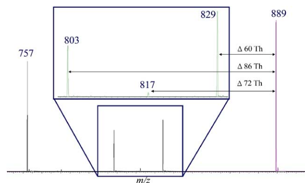
Figure 3. CID spectrum of \text{Na}^+ cationized \text{CH}_3\text{-PLA-O}(\text{C}=\text{O})\text{CH}_3 ( m/z 889; argon collision gas; 45 eV collision energy).
